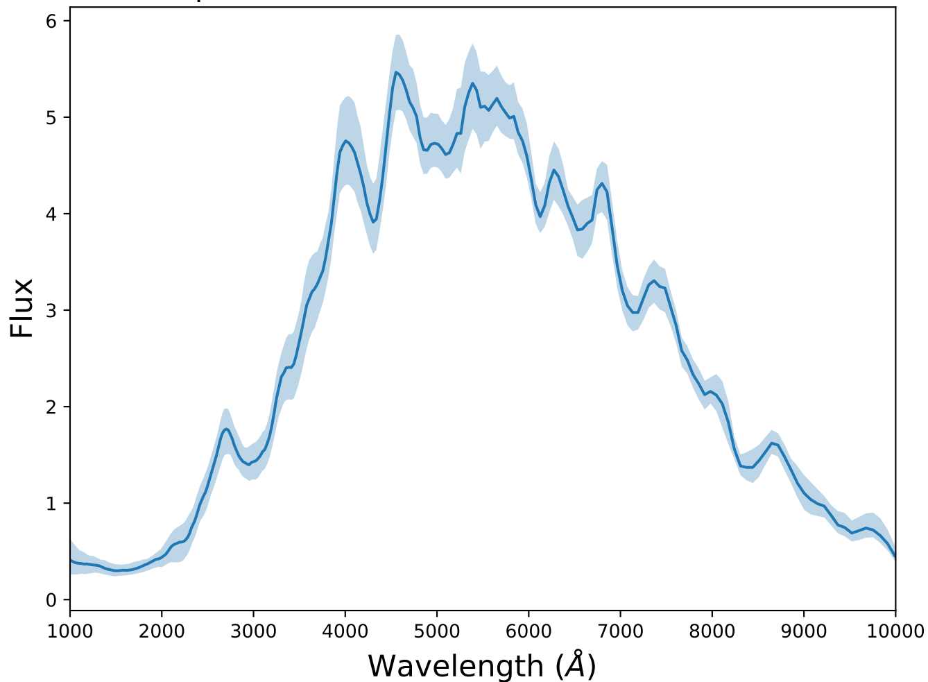
Spectrum 1 for transient SNIax at z=0.68
